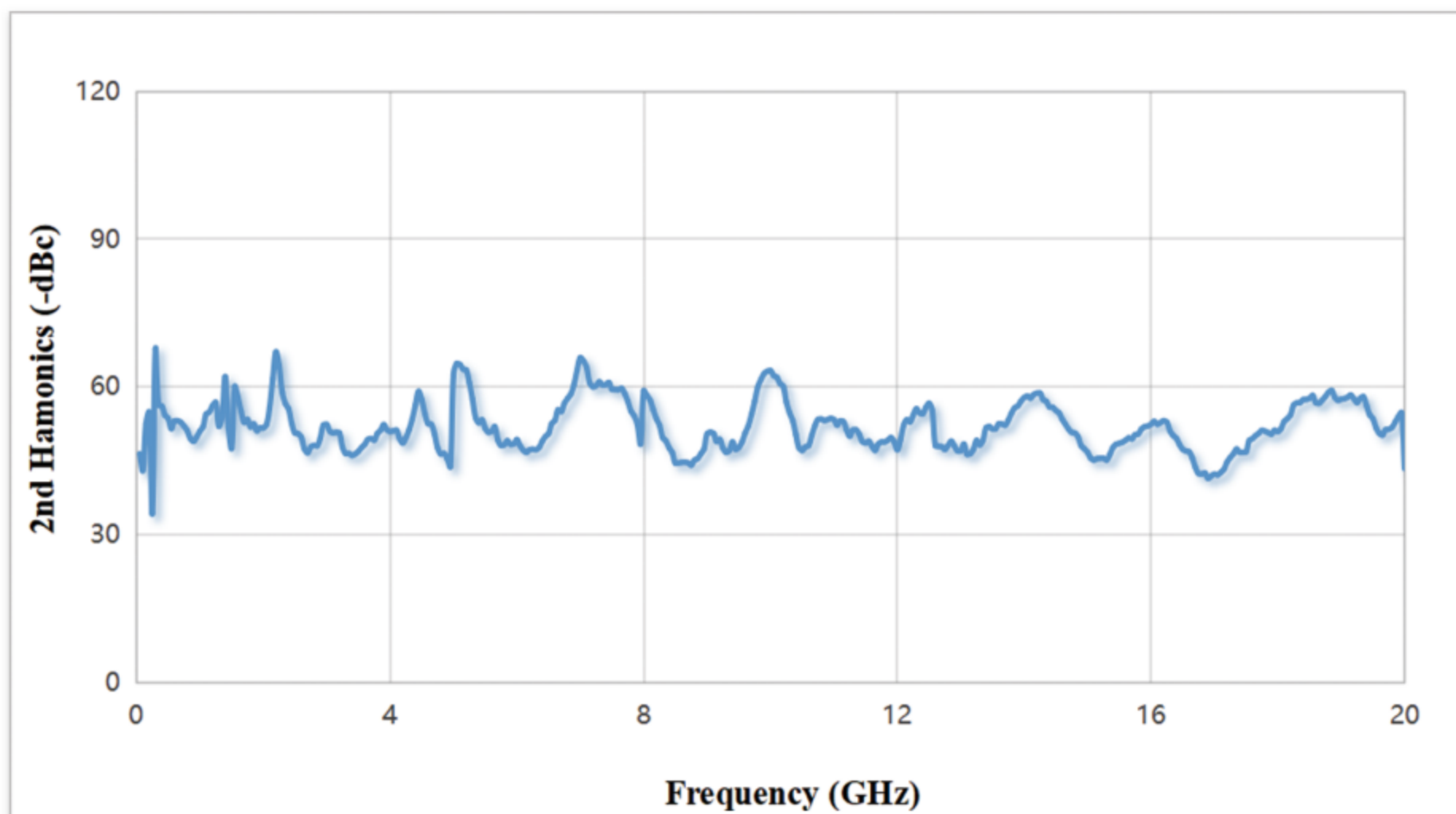
Output Power: +10dBm
