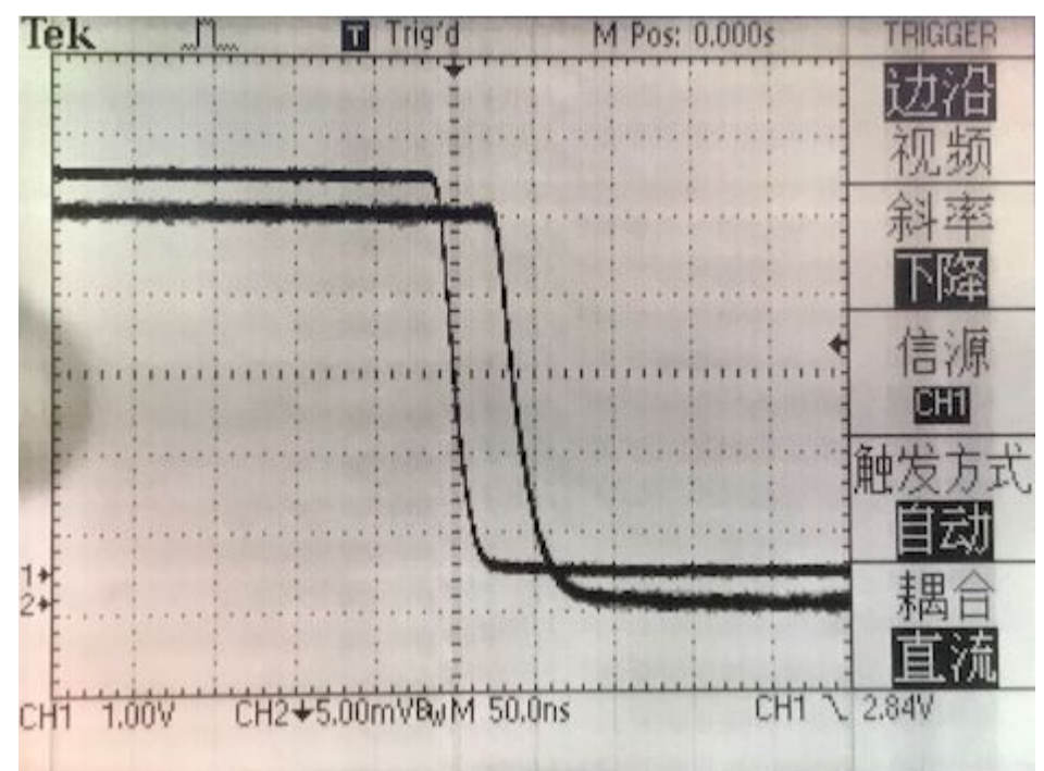
Turn Off Switching Speed
